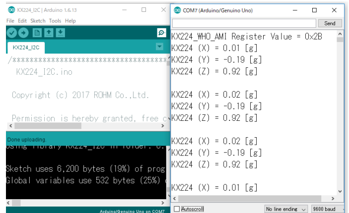
Figure 6. Serial Monitor 画面
