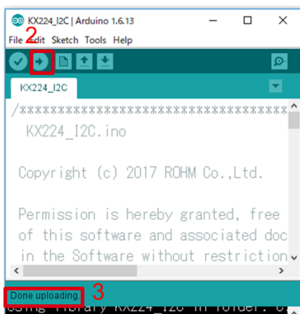
Figure 4. Upload 画面
