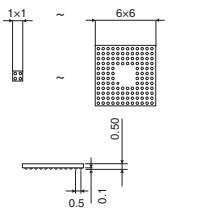
VCSP50L
