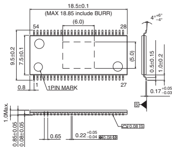
HTSSOP-B54
