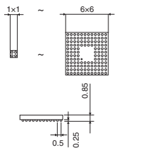
VCSP85H
