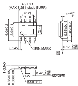
HTSOP-J8
