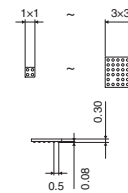
VCSP30L
