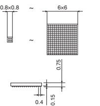
UCSP75M
