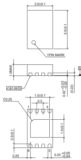
VSON008V2030
