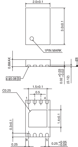
VSON008X2030
