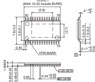
HTSSOP-B30
