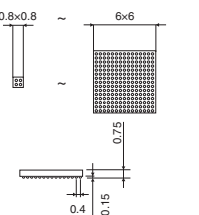
UCSP75M
