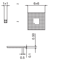
VCSP50L
