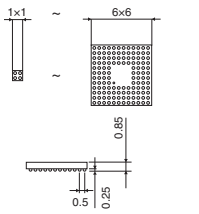
VCSP85H
