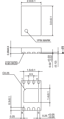
VSON008X2030
