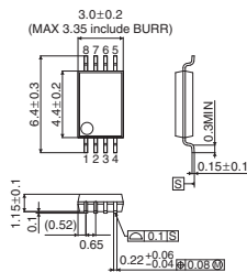
SSOP-B8
