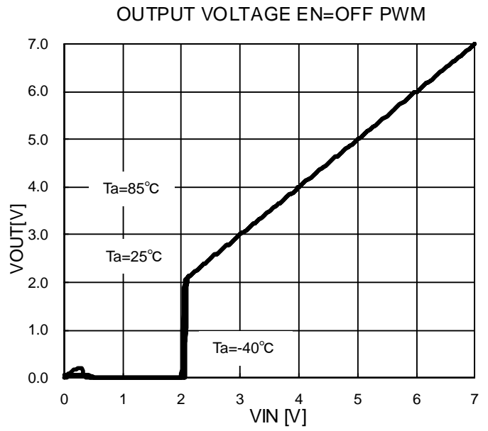
Figure 6. Out Put Vltage (EN=OFF) PWM
