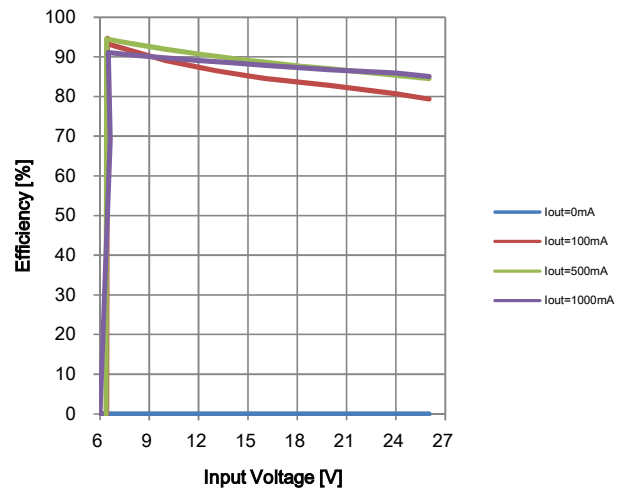
Figure.13-2 LINE Regulation (Efficiency: BP5293-50)
