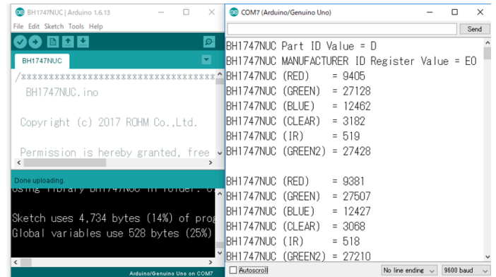
Figure 6. Serial Monitor 画面
